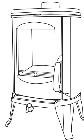
Sirius
